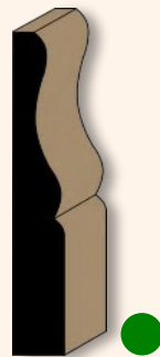
B-8 BASE 3-1/4"
